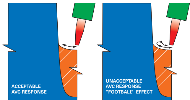
Figure 3. Acceptable and unacceptable AVC response. AVC setting must allow for flat weld bead placement without humping.
