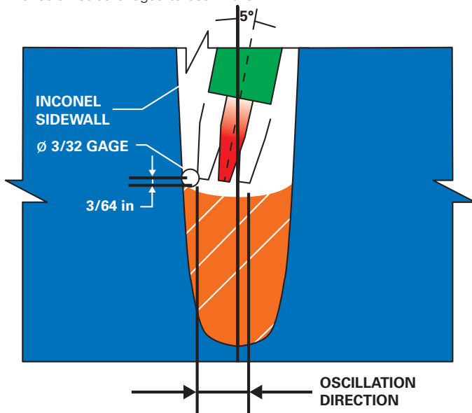
Figure 4. A gauge is used to set the distance between the tungsten electrode and the sidewall.
