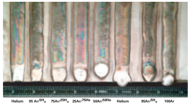
Figure 6. The effect of various shielding gas mixtures on weld bead shape and appearance for cladding applications.
