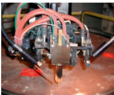
Figure 1. A narrow gap torch mounted on an Arc Machines, Inc. weld head in a Model 2 fixed automation system with remote wire positioning, remote torch tilt and leading and trailing cameras.
