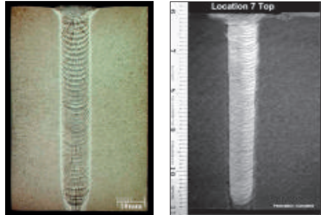
Figure 2. Macrographs of welds performed with a narrow gap torch. Left: Weld bead deposited using a single bead per layer technique in the 5G position. Right: Weld beads deposited using a two bead per layer technique in the horizontal position. This technique results in more favorable grain structure.
