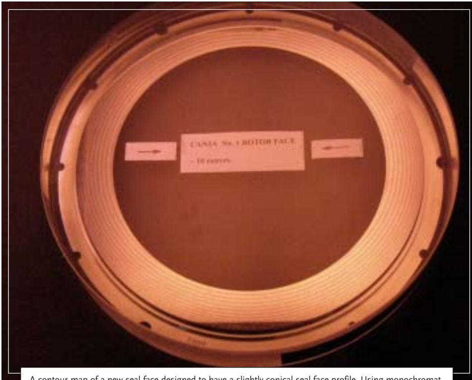
A contour map of a new seal face designed to have a slightly conical seal face profile. Using monochromatic light through an optical flat (an extremely flat piece of quartz glass) an interference pattern is produced showing the flatness of the face. The convexity (i.e., the difference in height of the inside of the face relative to the outside) is roughly 9 lightbands, or 4 \mu\text{m} . After a seal has been run, the face is usually roughened slightly and the lightband patterns are no longer visible.
